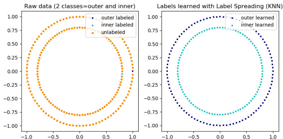
Fig. 1: An illustration of label-propagation: the structure of unlabeled observations is consistent with the class structure, and thus the class label can be propagated to the unlabeled observations of the training set.
