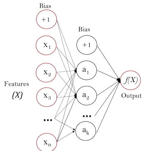
Fig. 2: Figure 1 : One hidden layer MLP.
