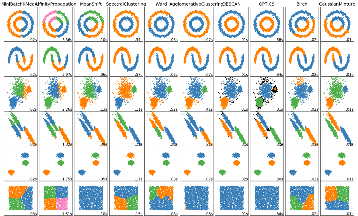
Fig. 4: A comparison of the clustering algorithms in scikit-learn
