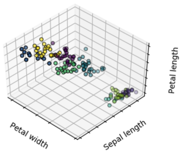
8 clusters
