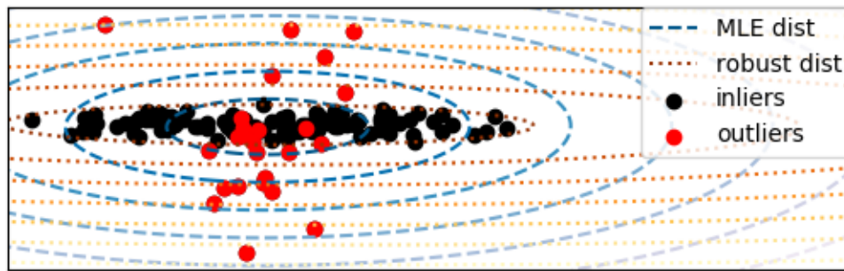
Mahalanobis distances of a contaminated data set:
