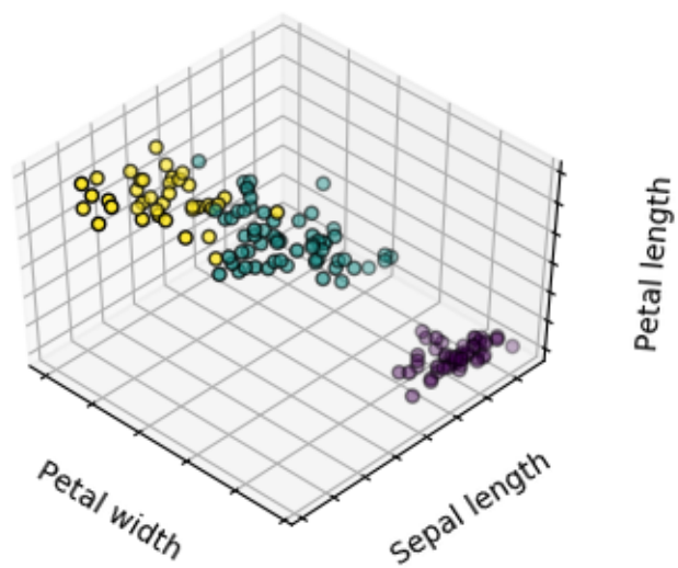
3 clusters
