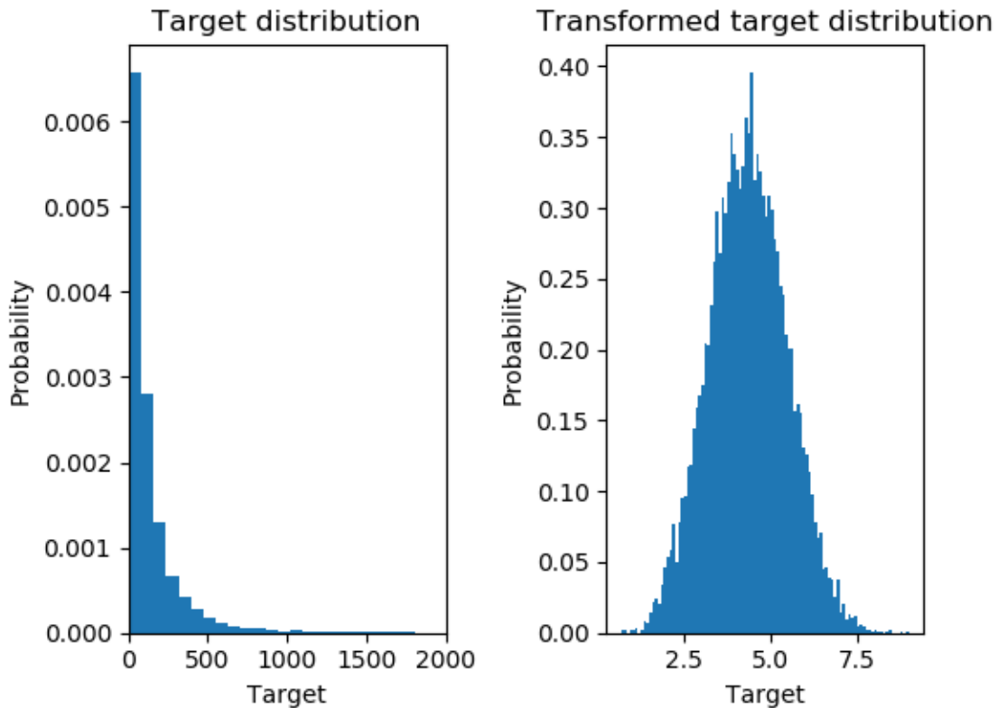
Synthetic data
