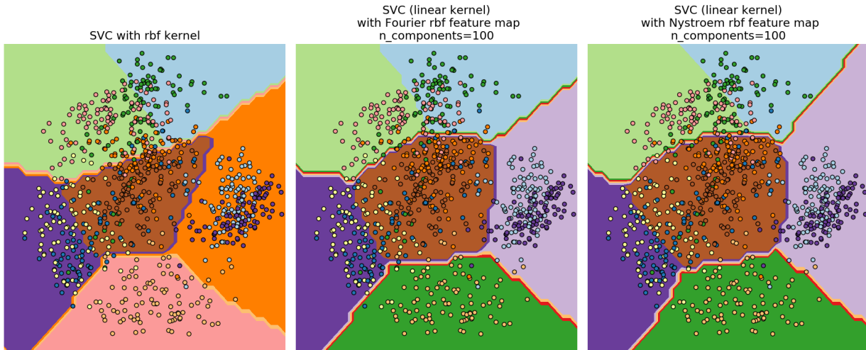
Fig. 9: Comparing an exact RBF kernel (left) with the approximation (right)
