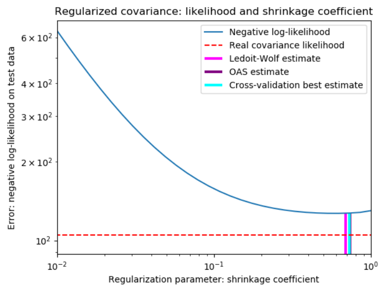
Fig. 7: Bias-variance trade-off when setting the shrinkage: comparing the choices of Ledoit-Wolf and OAS estimators
