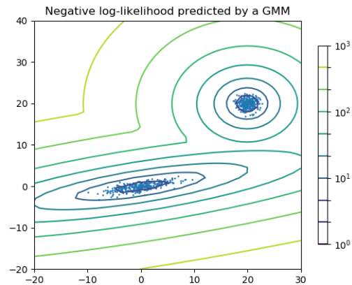
Fig. 3: Two-component Gaussian mixture model: data points, and equi-probability surfaces of the model.
