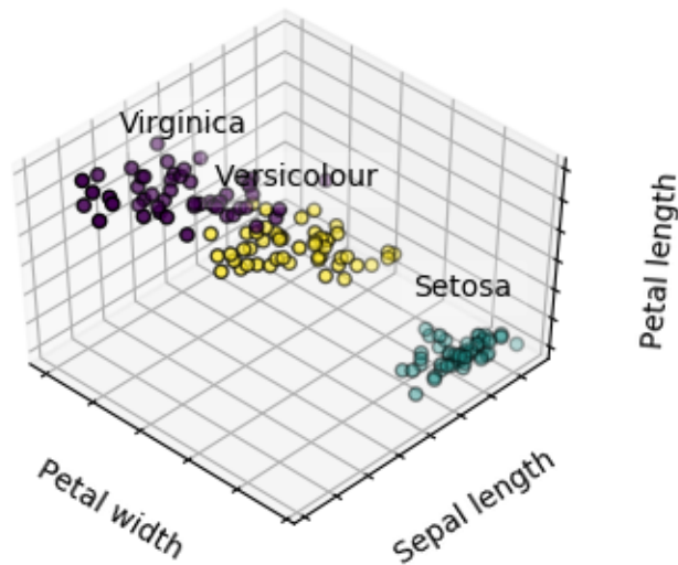
Ground Truth
