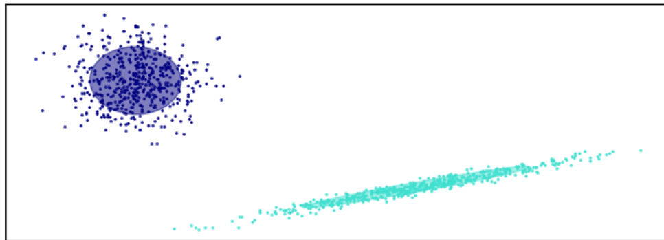
Selected GMM: full model, 2 components
